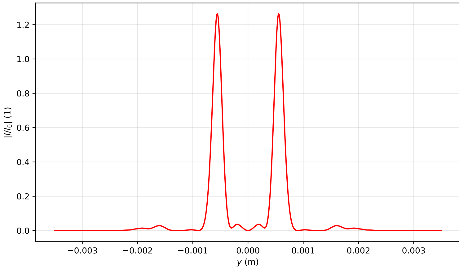
Intensity profile I(x=0, y, z=1.433)/I_0 , P_{in}=9.0P_{cr} , artificial time
